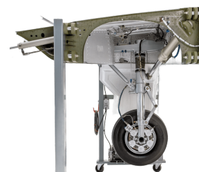
Landing Gear
